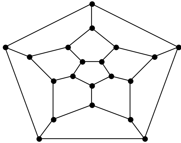
Dodecahedron
