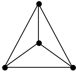
Tetrahedron ( K_4 )
