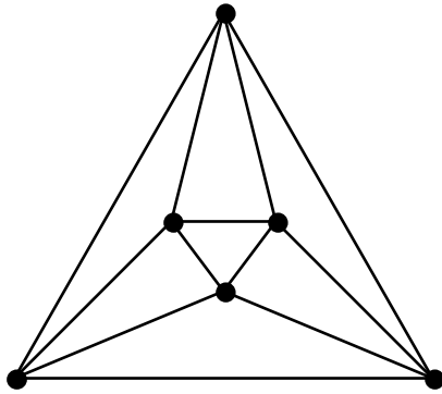
Octahedron
