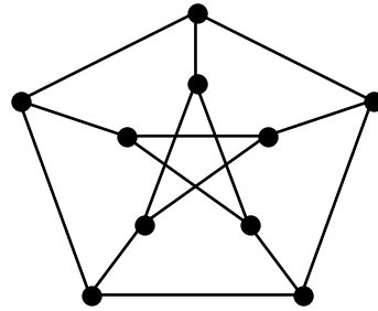
Petersen's graph
