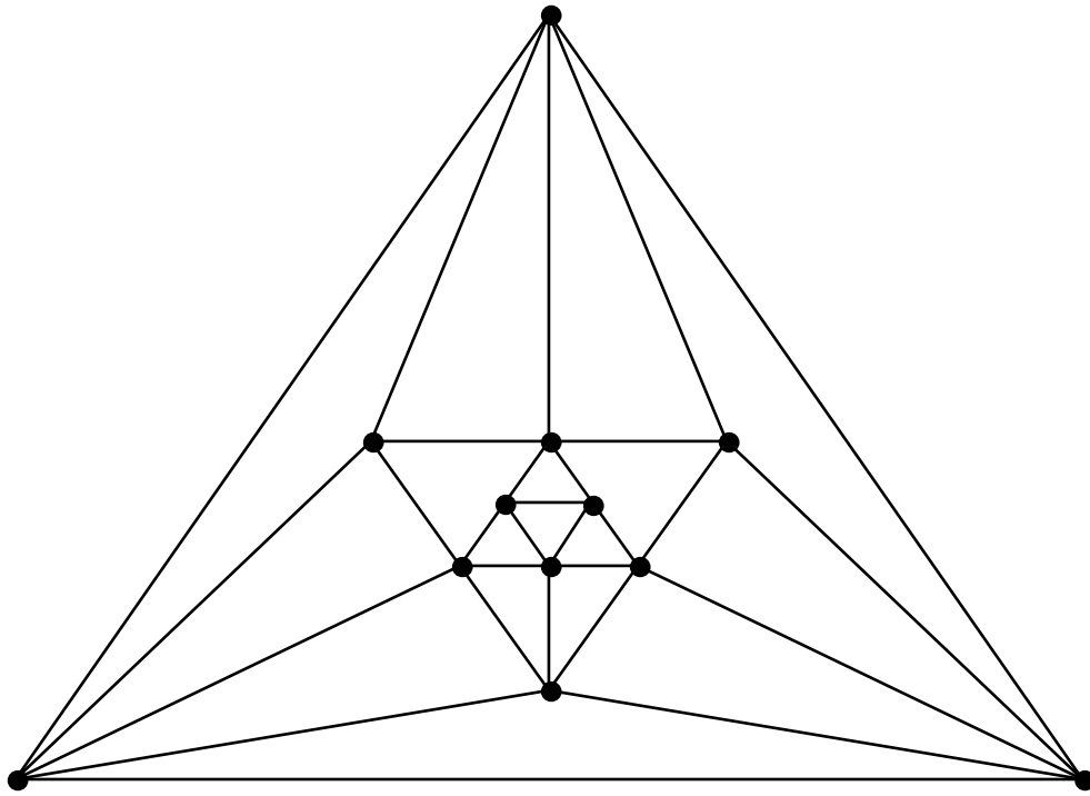
Icosahedron
