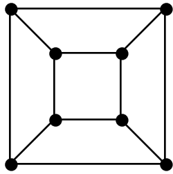
Cube graph
